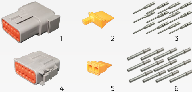
40.01mm W x 20.22mm H x 43.69mm L DTM04-12P
